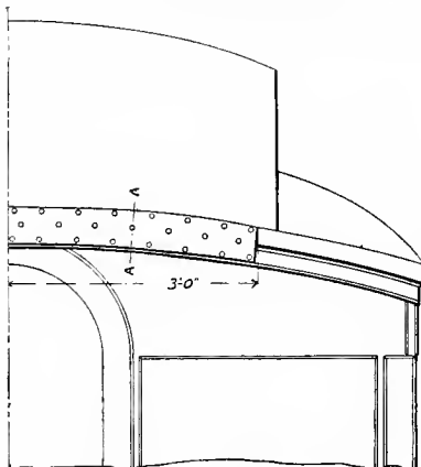
Fig. 2446. Hood-carcine Face-plate. Applied to cars with vestibules to prevent diaphragm face-plate from crushing hood-carcine.
